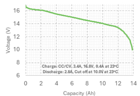
Discharge Characteristics:
