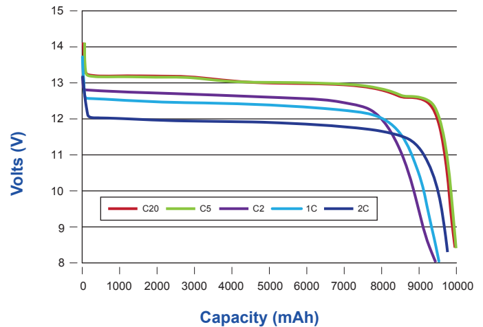
K2B12V10 at Different Discharge Rates
